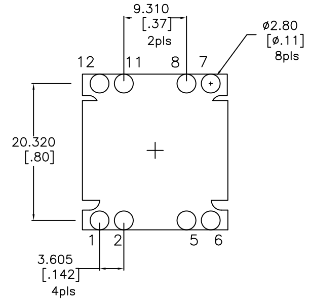
SUGGESTED PAD LAYOUT [PCB TOP VIEW]
