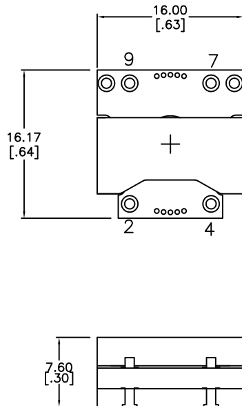
MECHANICAL [TOP VIEW]
